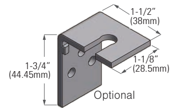
Optional KT151 hanger adapter bracket, face-mounted on door
